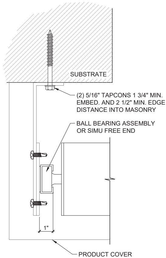
CUSTOM HOOD / BRACKET WALL MOUNT
