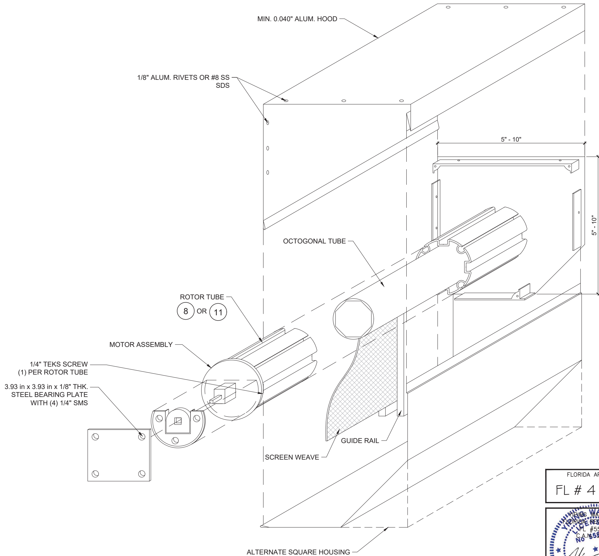
HOUSING ASSEMBLY DETAIL - OPTION NOT PART OF THIS APPROVAL
